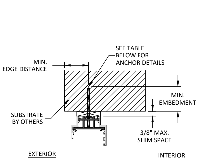
A 6 VERTICAL SECTION HEAD - THROUGH FRAME
